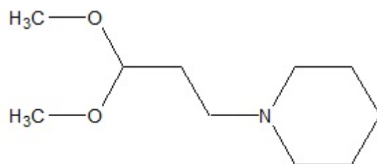
1-Piperidinepropionaldehyde dimethyl acetal
